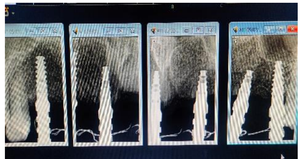
RADIOGRAPHS OF JIG TRIAL
